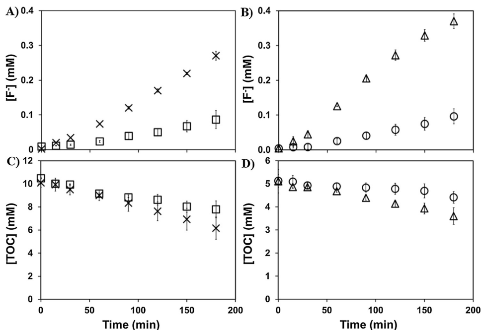
Fig. 3. Sound frequency effect on the sonochemical degradation of 929.4× dilution AFFF. This figure shows as a function of the sonication time (180 min) the release of fluoride when 3M (panel A) was sonicated under 500 kHz (□) or under 1 MHz (×); and when Ansul (panel B) was sonicated under 500 kHz (○) or under 1 MHz (Δ).
