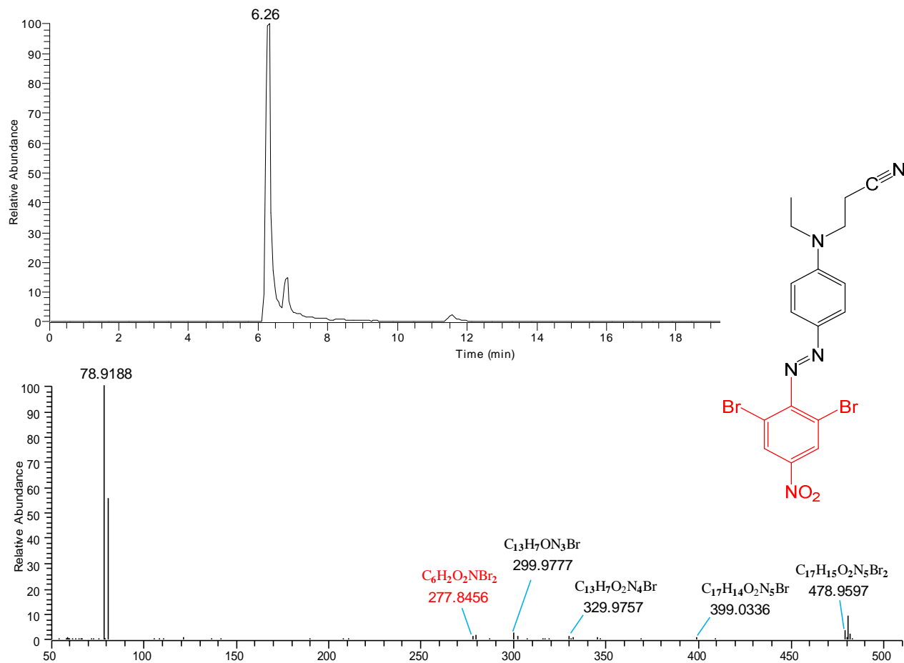
114 Figure S2. Chromatographic profile and MS/MS spectrum of a compound whose formula was 115 predicted to be \text{C}_{17}\text{H}_{15}\text{O}_2\text{N}_5\text{Br}_2 ( m/z = 478.9597 ). Database search suggested Disperse Orange 61 116 (structure shown in the figure) as a probable candidate. Fragment ions commonly observed for a 117 brominated azo dye, especially the fragment ion resulting from the breakage of bond between 118 azo nitrogen and aromatic ring (shown in red) indicate the compound likely to be a Disperse 119 orange 61.
