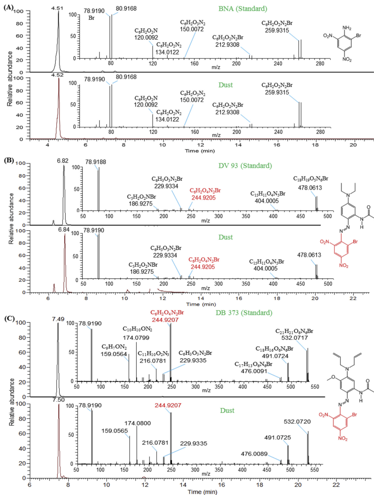
Fig. 1. Identification of (A) 2-bromo-4,6-dinitroaniline (BNA), (B) Disperse Violet 93 (DV93), and (C) Disperse Blue 373 (DB373) in a dust sample by comparing chromatographic congruence and fragmentation with synthetic standards. (For interpretation of the references to color in this figure legend, the reader is referred to the Web version of this article.)
