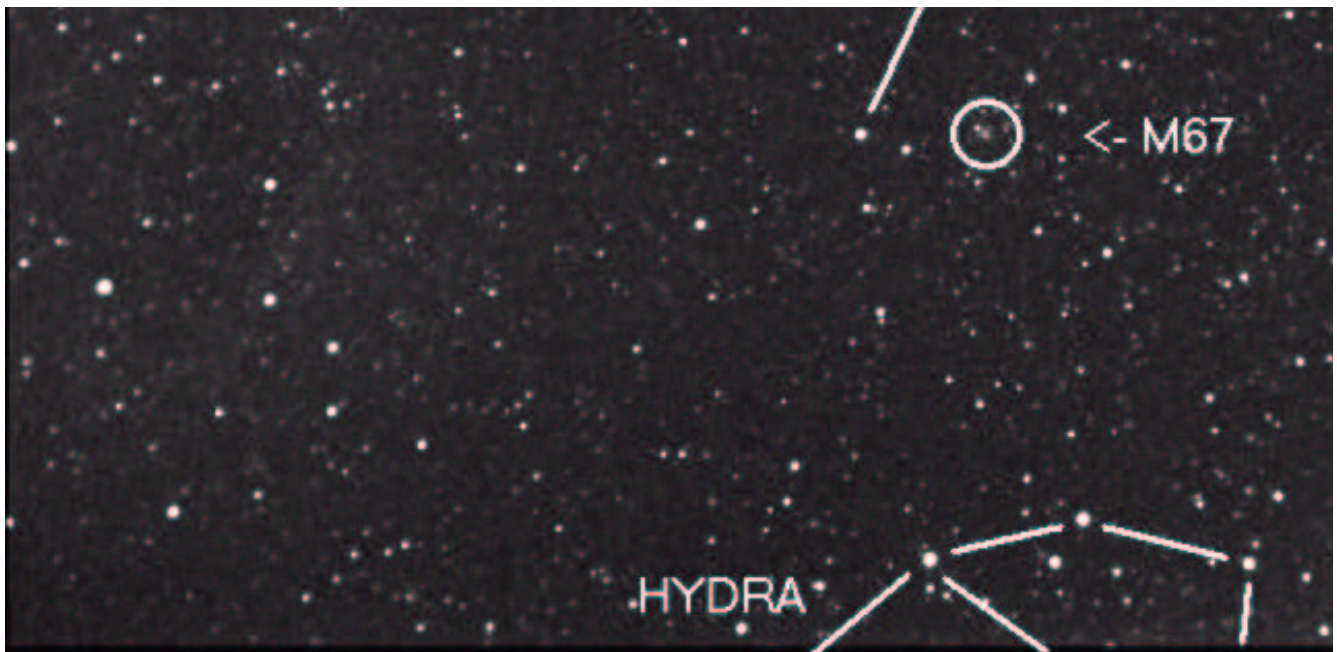
Figure 13. Southern part of the constellation Cancer. M67 is a "smudge" at this resolution (160 "arc). The image is 21.3 degeres across.
