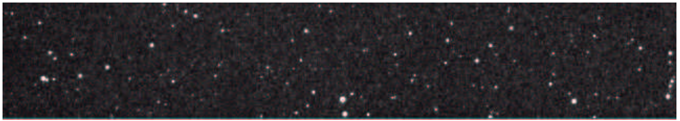
Figure 14. Zoom factor 1.5. Image size is 7.8 x 5.1 degrees. The faintest stars are 13.5 magnitude. [SBIG ST-8E, Nikon 100 mm EFL, f/11, median combine of twelve 30-second exposures; 2002.05.08.3 UT, Santa Barbara residence]
