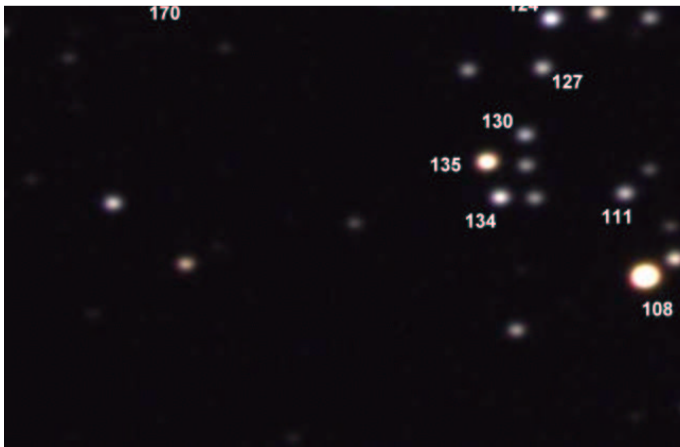
Figure 18. Zoom of central region of previous image. Star #135 has coordinates 8:51:22, +11^{\circ} 46' 06'' (epoch 2000.0). The image area is 6.82 \times 4.85' arc. The FWHM resolution is 4.0'' arc in this sum of several 1-minute unguided exposures using BVR filters. The faintest stars have a visual magnitude of about 14. Stars to be used by AAVSO observers are indicated with star numbers. The bluest star is #81 and the reddest is #108. [LX200 10-inch SCT, f/6.3, SBIG ST-8E, True Tech filter wheel w/ Schuler BVRI filters; 2002.04.22Z, Santa Barbara, CA.]
