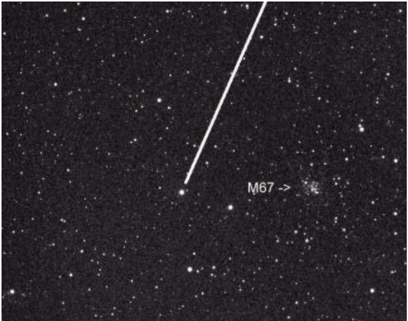
Figure 13. Southern part of the constellation Cancer. M67 is a "smudge" at this resolution (160 "arc). The image is 21.3 degeres across.
