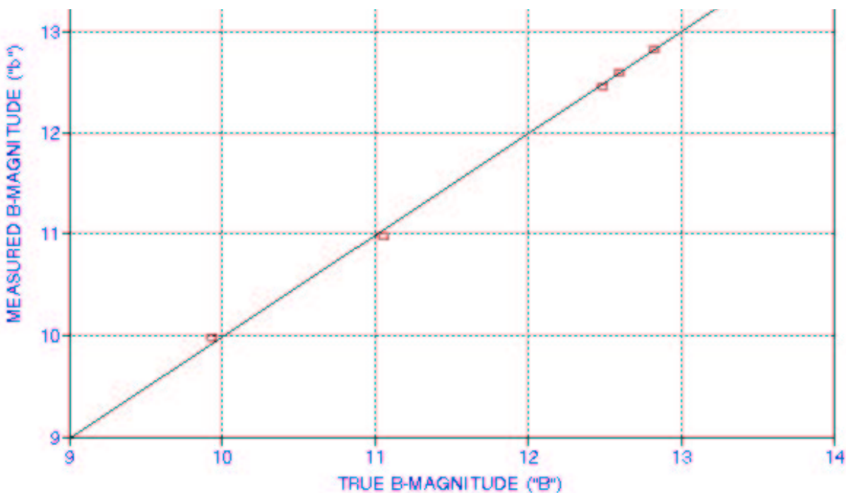
Figure 24. Plot of measured "b" magnitudes versus M67 comparison star "B" magnitudes using the "8E/Schuler" system.
