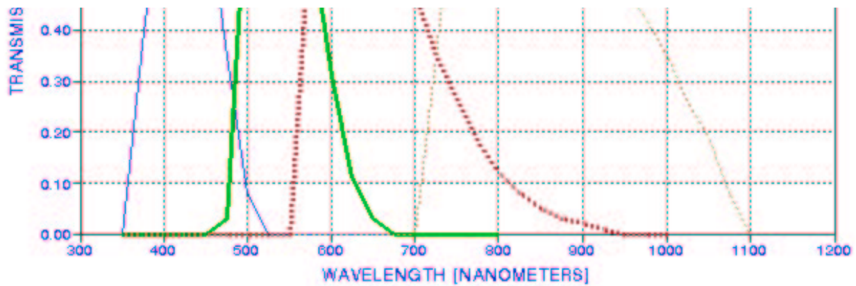
Figure 2. Typical BVRI filter spectral response (i.e., band pass).
