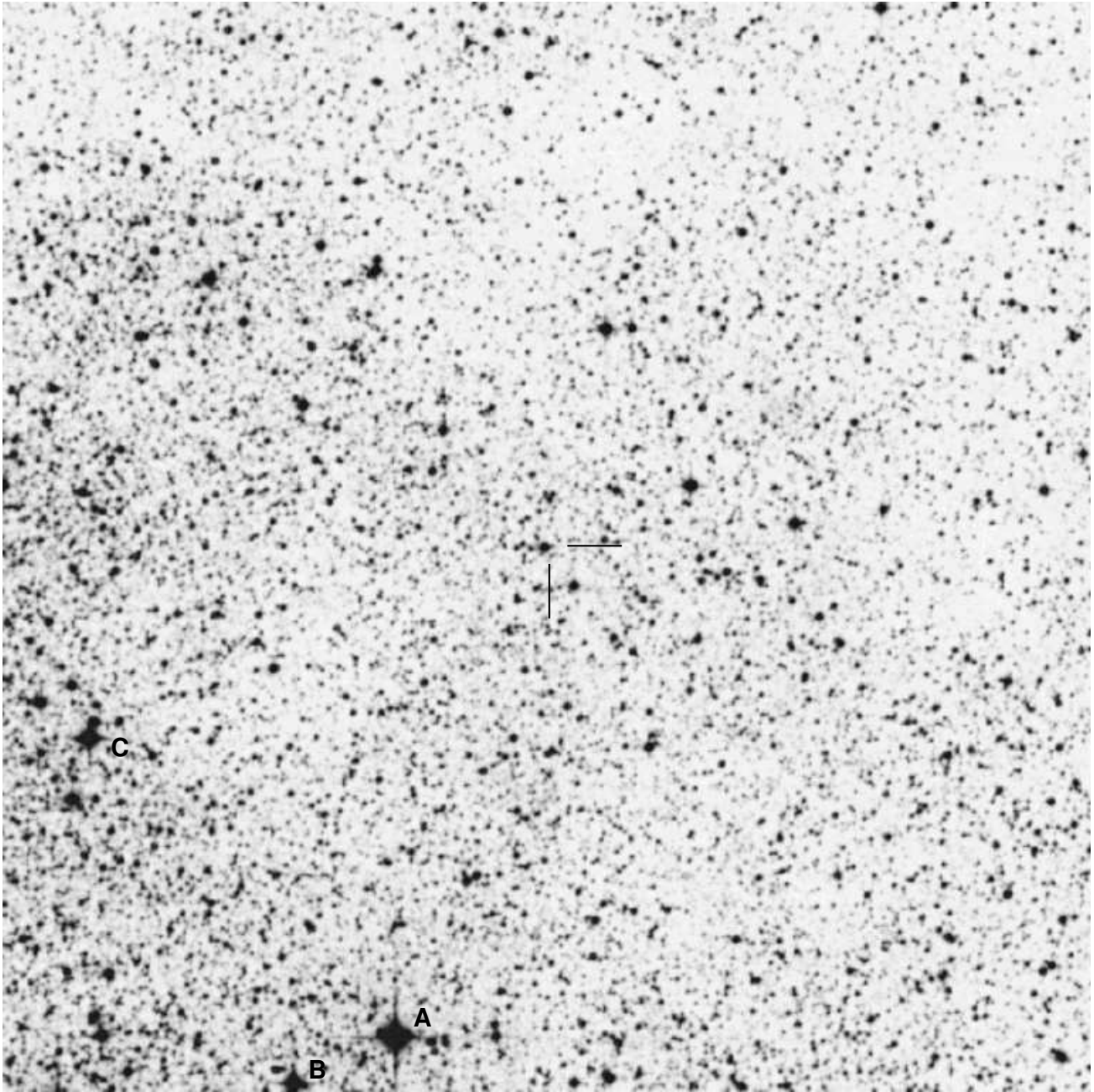
1845.0-0433: 18^h45^m01^s.5 -04^\circ33'55''.5 (J2000) V=13.96 15m ( 1/4^\circ ) sq field — North right, East down. In northern Scutum, Uranometria 250. Position from: Coe MJ et al. MNRAS 281, 333-338, 1996. O9.5I
