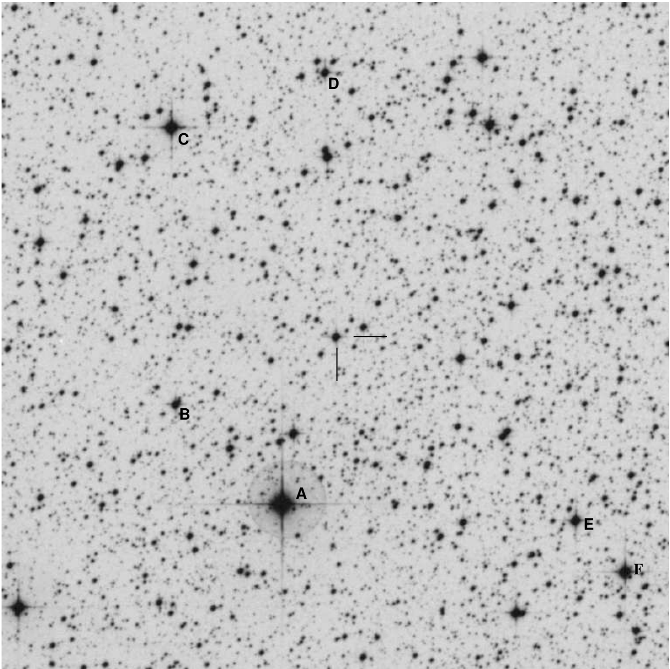
J1037.5-5647: 10^h 37^m 35^s.2 -56^\circ 47' 59'' (J2000) V=12.3 15m ( 1/4^\circ ) sq field — North right, East down. In Vela, Uranometria 427. Position from: Motch et al., Astron. Astrophys. 323, 853-875, 1997. B0V-IIIe, Probably same as LPH068 = 4U1036-56
